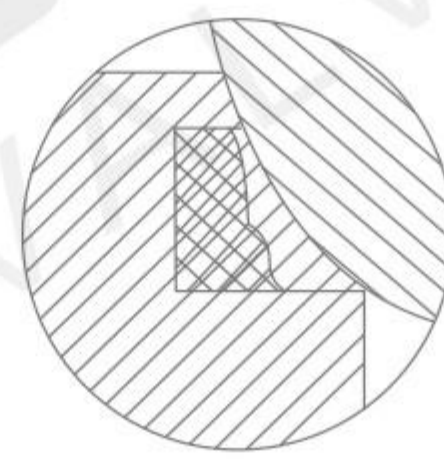
阀座耐火结构 Refractory structure of valve seat
