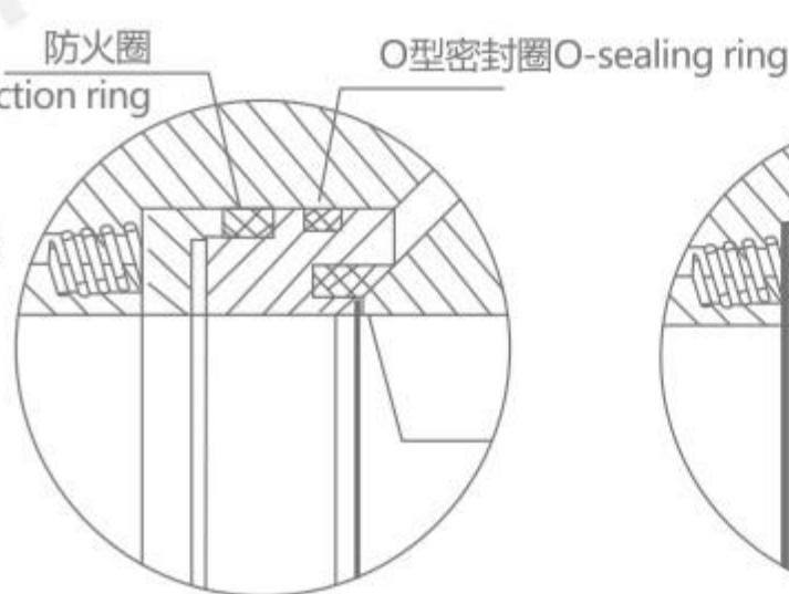
阀座耐火结构 Refractory structure of valve seat
